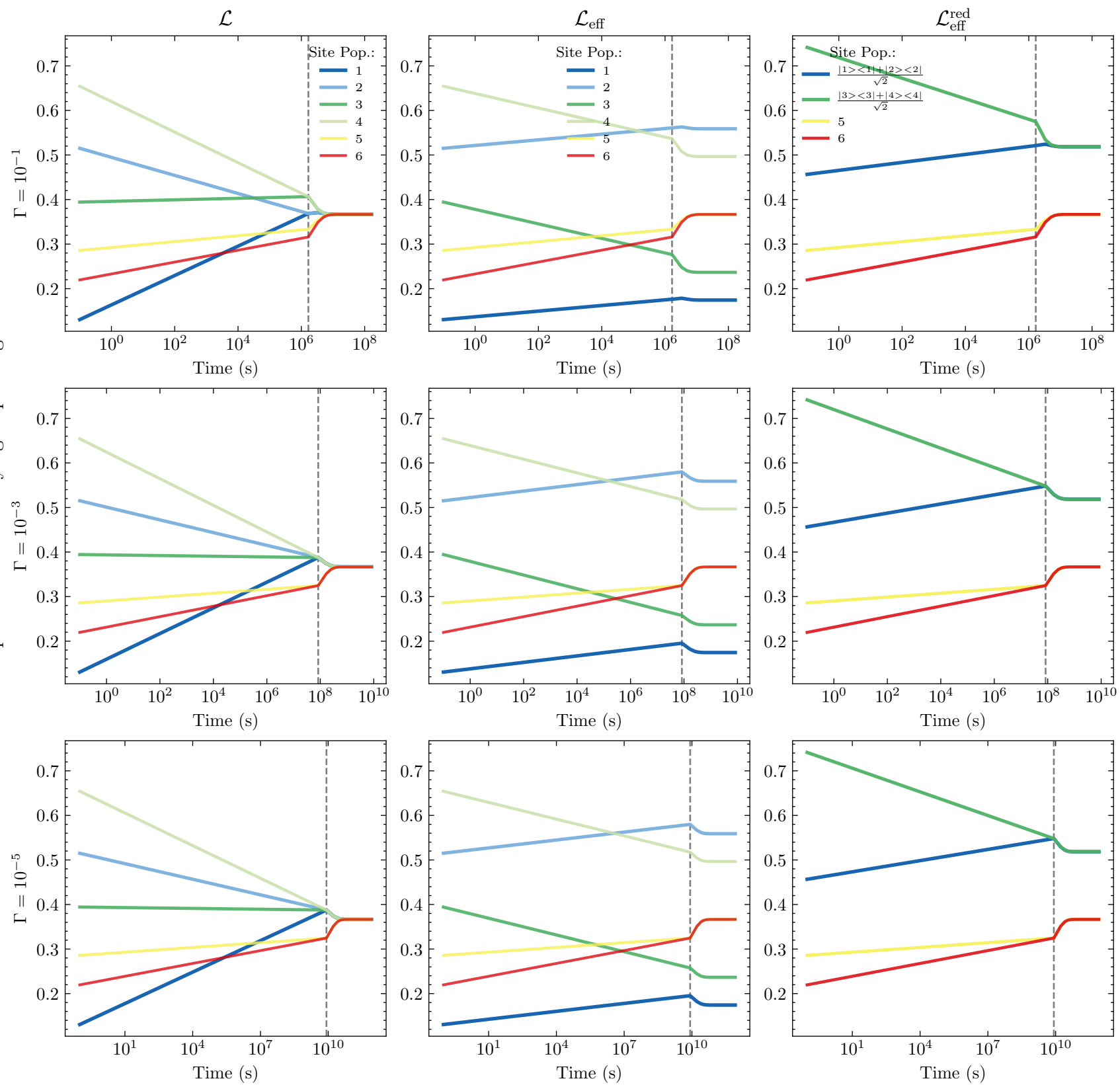
Time Evolution of Site Populations under \mathcal{L} , \mathcal{L}_{\text{eff}} , and \mathcal{L}_{\text{eff}}^{\text{red}} N=6 ; N_{\text{dimers}}=2 ; N_{\epsilon}=2 ; J = 10^{-1} ; \epsilon = 10^{-4} ; seed=185
